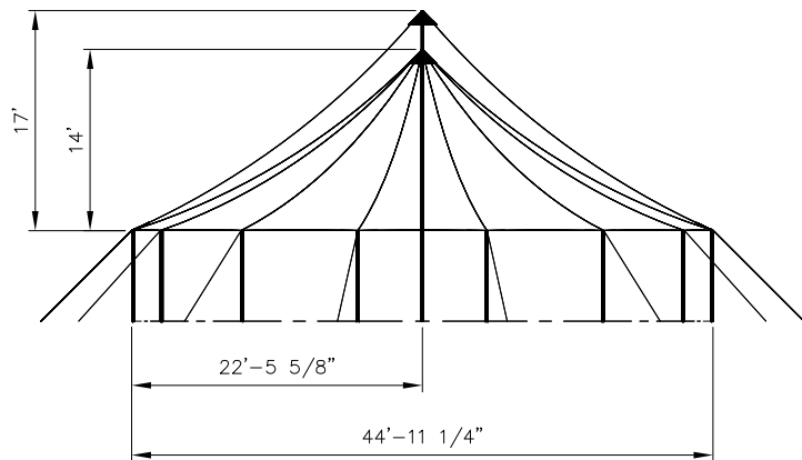
END VIEW
